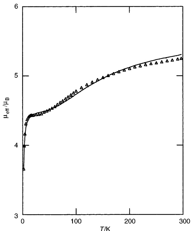
Fig. 3 Temperature dependence of the effective magnetic moments \mu_{\text{eff}} is calculated as 2.828 (\chi_{\text{m}} T)^{\frac{1}{2}} . The solid line represents the best fit of the theoretical susceptibility values to the experimental data
