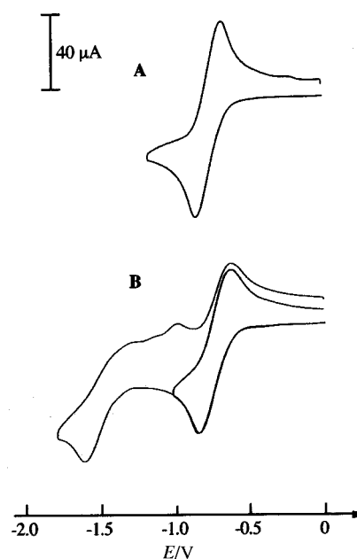
Fig. 4 The electrochemical behaviour of complexes 1 and 2 in \text{CH}_2\text{Cl}_2 + \text{NBu}^n\text{ClO}_4 (0.1 mol \text{dm}^{-3} ) using a \text{Ag}-0.01 \text{ mol dm}^{-3} \text{AgNO}_3 reference electrode and a glassy carbon disc as working electrode (diameter: 5 mm). Curves: A, a 2.3 mmol \text{dm}^{-3} solution of 1 ; B, a 2.2 mmol \text{dm}^{-3} solution of 2 , v = 0.1 \text{ V s}^{-1}
